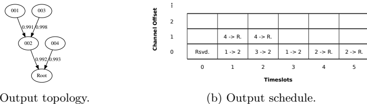
Fig. 4.8: Output topology and schedule for the 4 nodes network example. Taken from [88].
