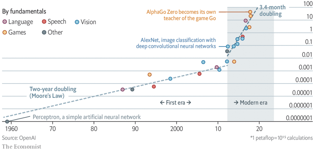
Figure 2.14: Compute capacity needed to train state of the art Deep Learning systems. Figure from The Economist, data from Open AI.
