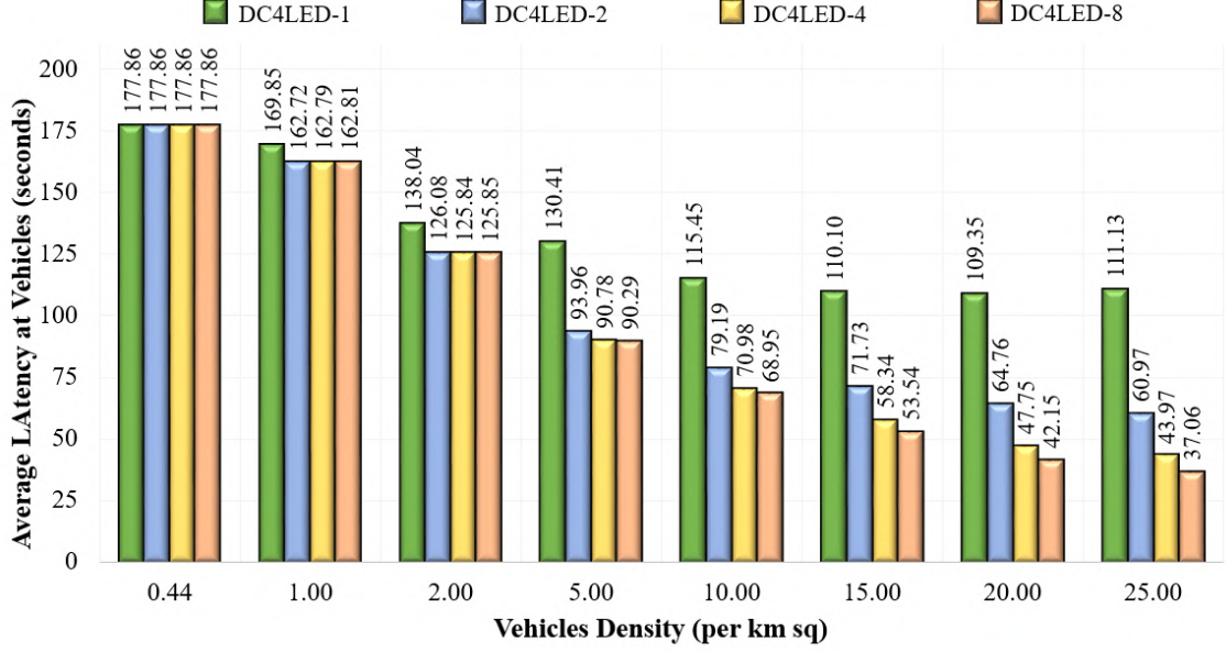
Figure 7.5 – The Average Latency at Vehicles
