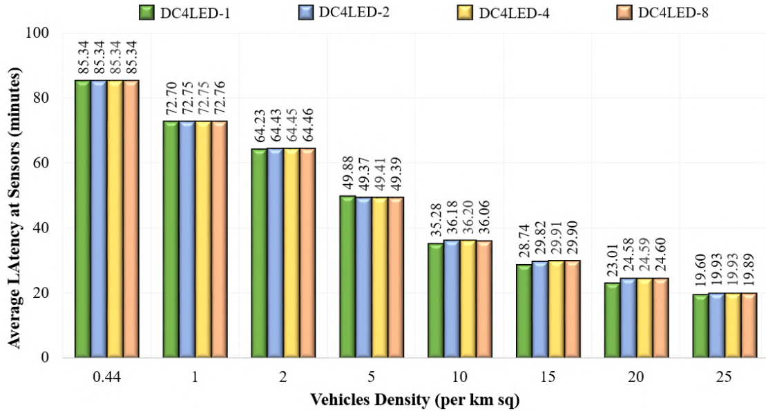
Figure 7.3 – The Average Latency at Sensors
