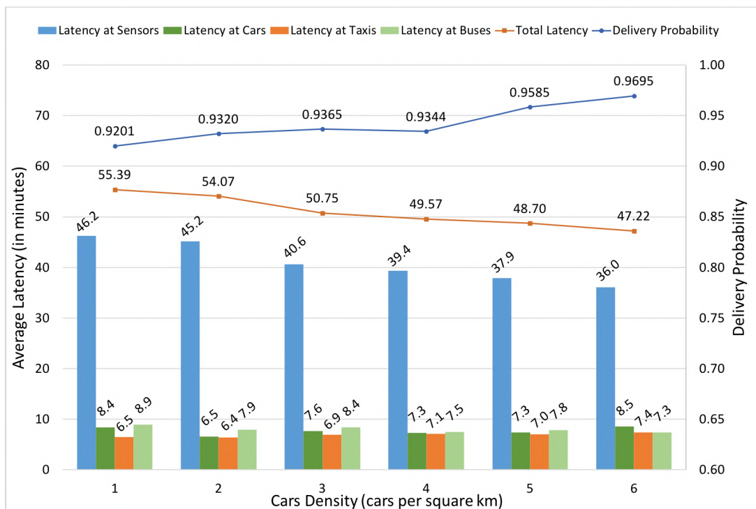
Figure 5.5 – The Delivery Probability and Average Latency
