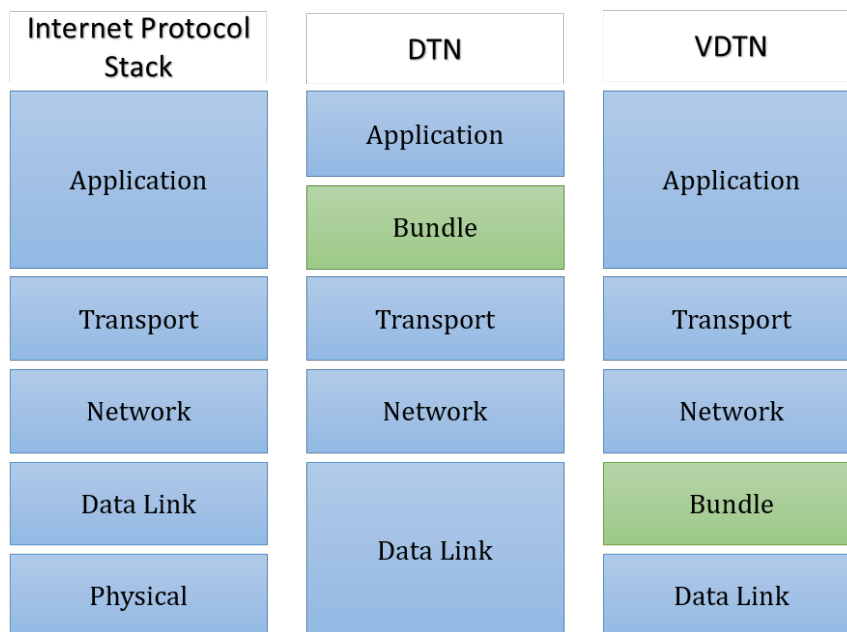
Figure 3.1 – Internet Protocol Stack, DTN, and VDTN Architecture
