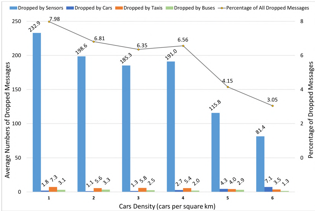
Figure 5.6 – The Dropped Messages Percentage and Distribution
