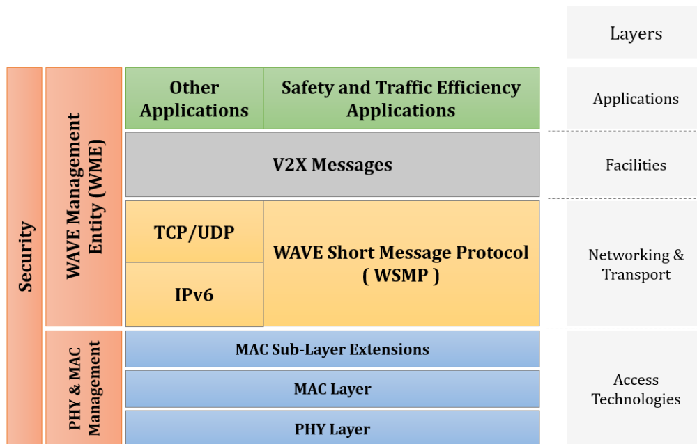
Figure 2.2 – DSRC Protocol Stack
