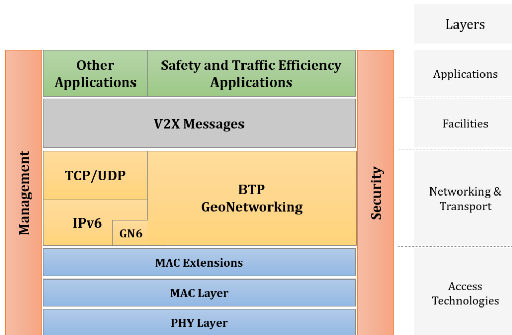
Figure 2.3 – C-ITS Protocol Stack
