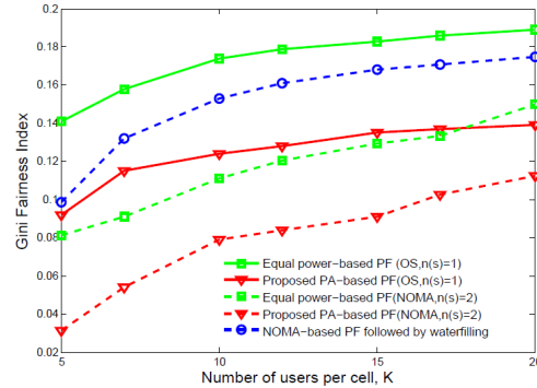
Fig. 3. Gini fairness index in terms of K , for 128 subbands.
