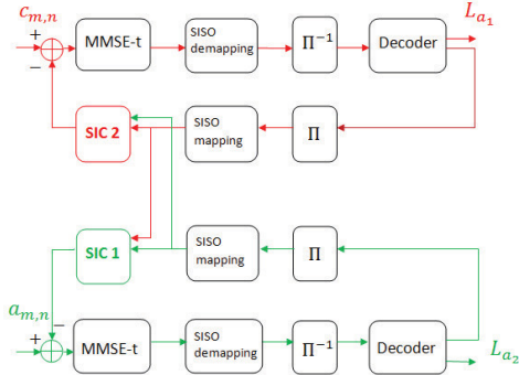
Fig. 3: Structure of the SISO MMSE LE-IC used for SIPC-tf.
