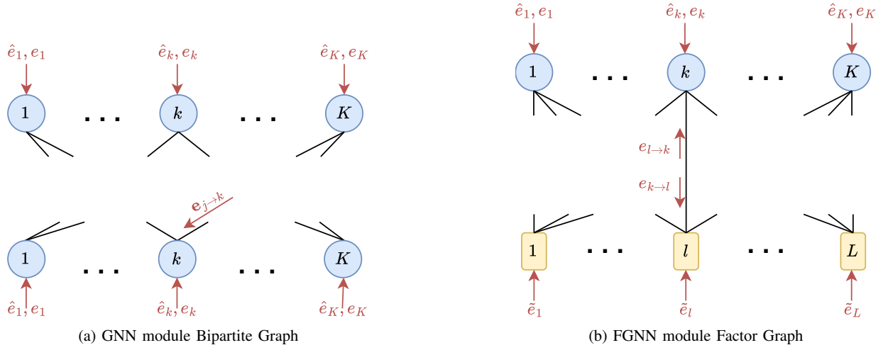
Figure 4.4: Two different graphical models of the MU-MIMO transmission
