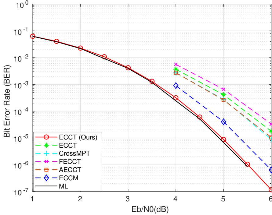
Figure 1.27: BER performance measured of our ECCT(128,6) model trained on BCH(63,45,7) with 64M ML error patterns generated following method 3 and compared to several reference transformer-based SBND models.
