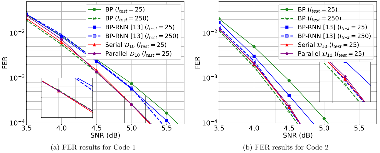
Figure 3.5: Frame Error Rate (FER) results
