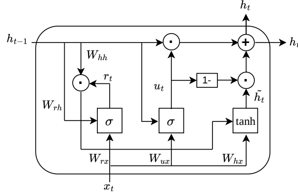
Figure 1.4: A typical structure of a GRU.
