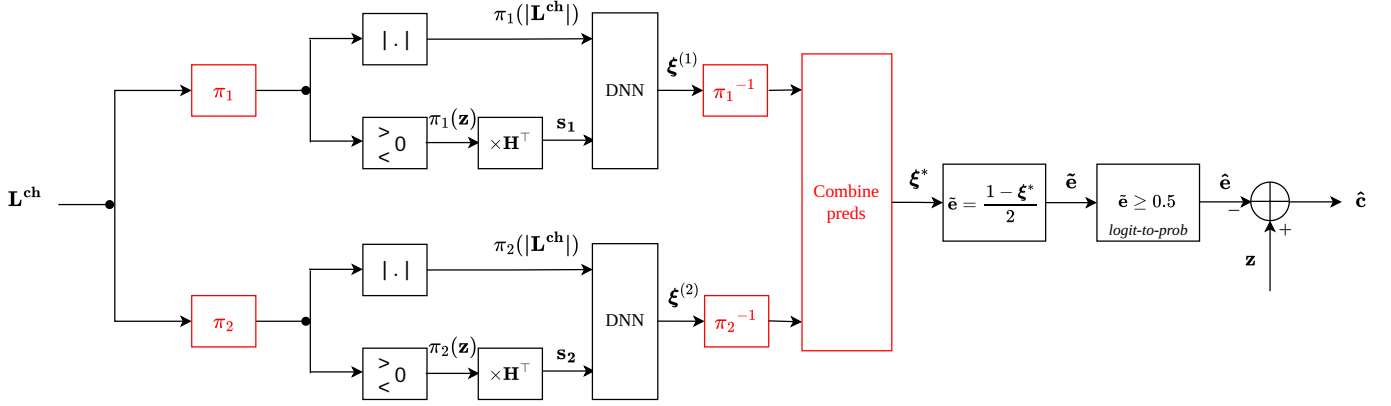
Figure 1.23: An illustrative diagram for the TTA process with T = 2 permutations.
