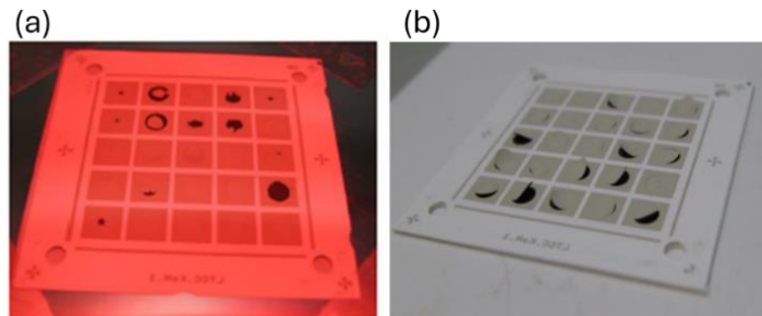
Fig. 4. (a) Metallization default after screen printing process, (b) Metallization removal problem and ferrite detachment during the drying phase.
