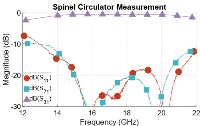
Fig. 12. Measured performances of the soldered Spinel circulator
