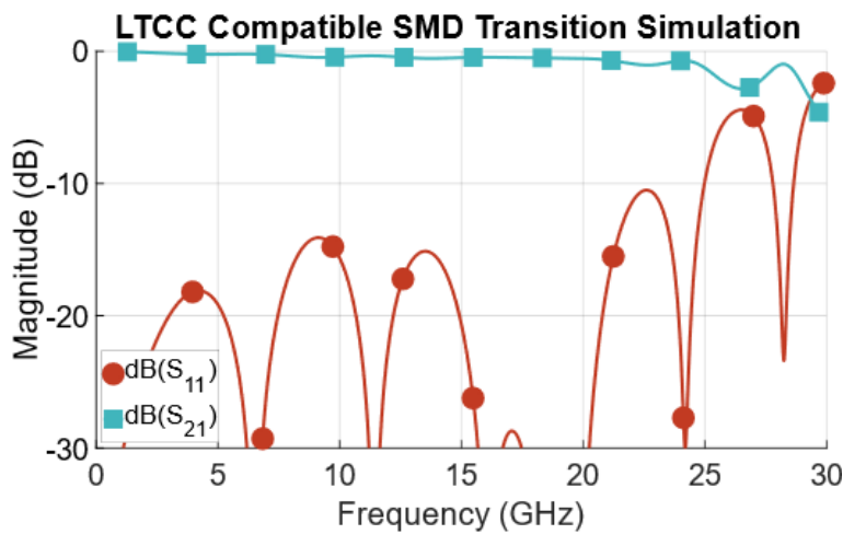
Fig. 4. SMD transition using a metallized half-via
