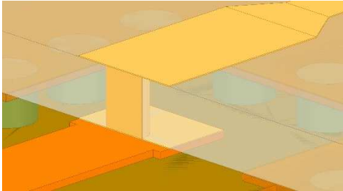
Fig. 2. SMD transition using a metallized half-via
