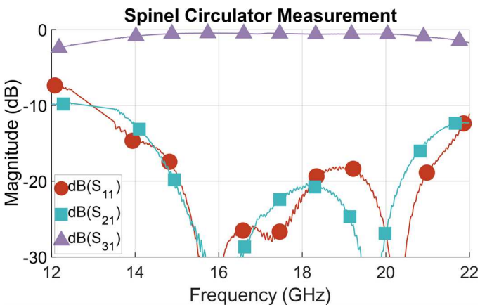
Fig. 12. Measured performances of the soldered Spinel circulator
