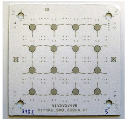
Fig. 8. Screen printing of the Y-junctions after the lamination step
