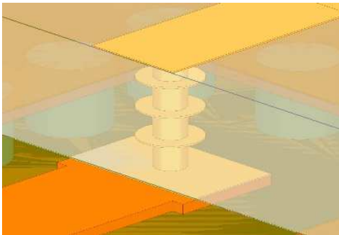
Fig. 3. SMD Transition compatible with the LTCC technology
