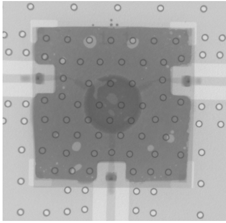
Fig. 10. X-ray observation of the soldered circulator
