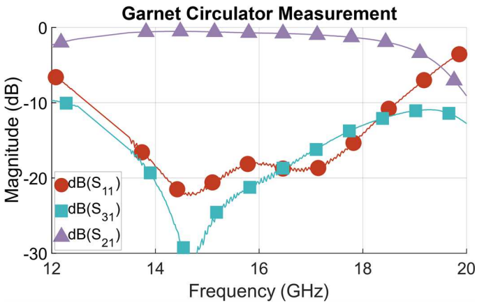
Fig. 11. Measured performances of the soldered Garnet circulator
