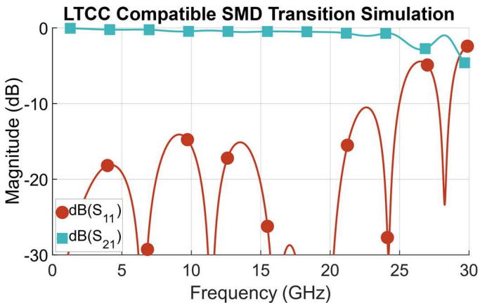
Fig. 4. S parameters of the LTCC compatible SMD transition
