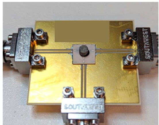
Fig. 9. Soldered circulator
