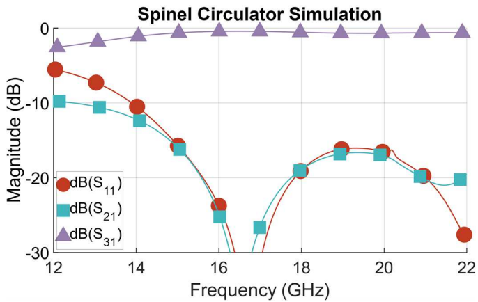
Fig. 6. Spinel SMD circulator simulation
