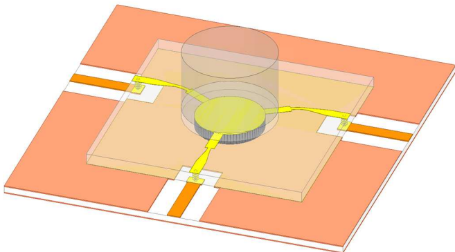
Fig. 1. SMD compatible LTCC circulator and the PCB
