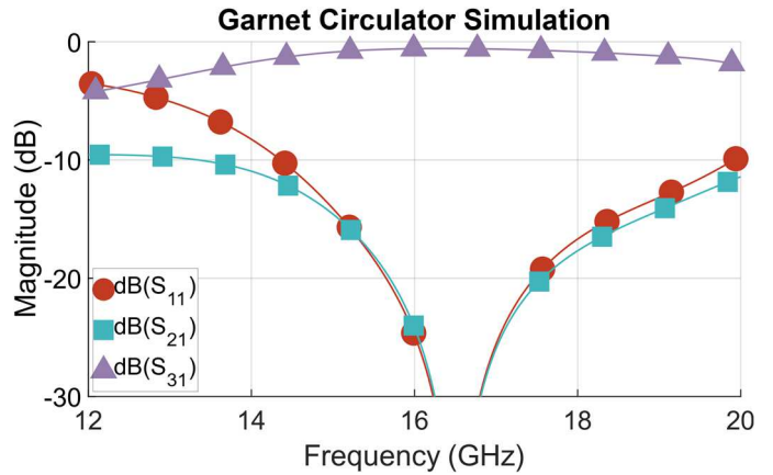
Fig. 5. Garnet SMD circulator simulation
