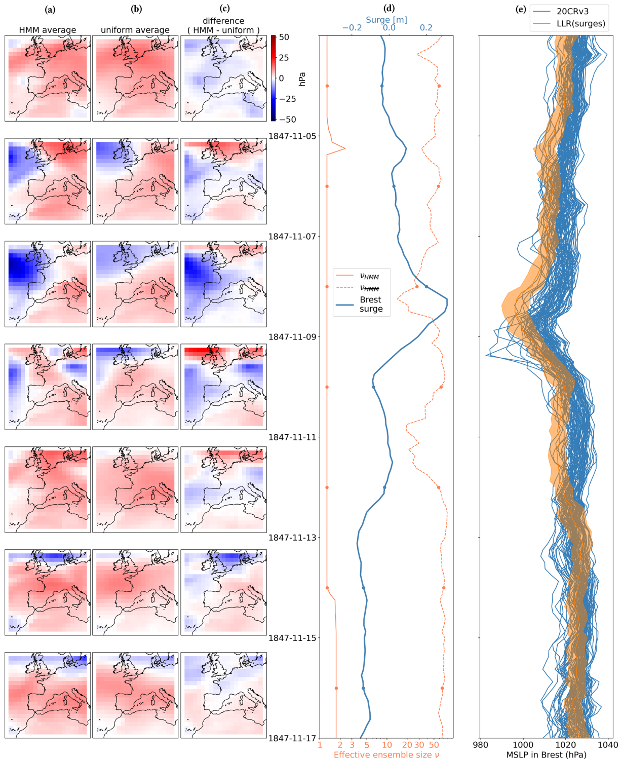
Figure 10. Mean result of the HMM algorithm in November 1847. (a) Average according to surge residual observations and HMM smoothing algorithm (probabilities p_{HMM}(i, t) ). (b) Average using constant uniform weights on 20CRv3 members. (c) Difference between HMM and uniform results. (d) Surge residual observations and effective ensemble sizes. (e) MSLP in Brest from ensemble members (blue lines) and local linear regression from surge residuals as an average \pm 1 SD (standard deviation). The dates of the left-hand plots are indicated with dots in (d) and (e) .
