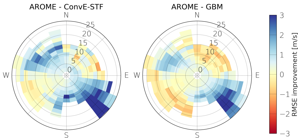
FIG. 12. RMSE improvement between ConvE-STF, gradient boosting machine (GBM) and AROME. The RMSE improvement ( RMSE(AROME) - RMSE(model) ) is shown in color, with blue sectors indicating a RMSE decrease compared to AROME, and red sectors a RMSE increase. The RMSE improvement is plotted as function of wind direction and wind speed.
