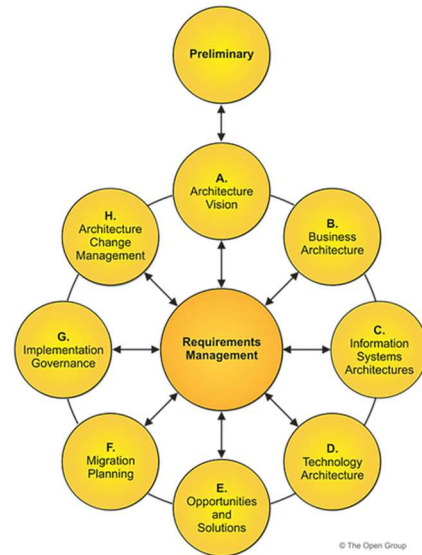
Figure 1. Structure of the TOGAF Architecture Development Method.
