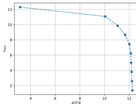
Figure 6. 10 solutions of a Pareto front.
