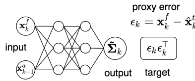
FIGURE 1 ANN training scheme. The training error is determined by the Frobenius norm between \tilde{\Sigma}_k and the training matrix \epsilon_k \epsilon_k^\top which is estimated from the approximated forecast error.
