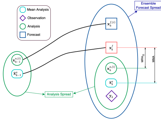
FIGURE 4 Schematic of an ensemble assimilation cycle where MRA and MMA forecast error proxies are shown using only the i -th ensemble member.
