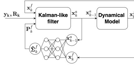
FIGURE 2 Schematic representation of an UnnKF assimilation cycle (see the text for details).
