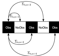
FIGURE 9 Pattern of observed (Obs) and unobserved (NoObs) state variables during data assimilation process and how each covariance ( \Sigma_{n,i} ) propagates information from one variable ( n ) to another ( i ).
