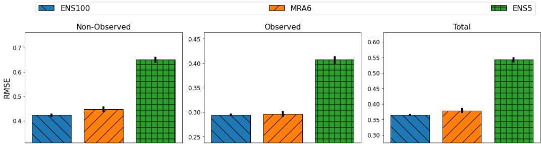
FIGURE 6 RMSE of the analyses generated by a 5-member ensemble (ENS5), a 100-member ensemble (ENS100) using ENKF method and the UnnKF method (MRA6) for the 100-variable Lorenz'96 model. The RMSE of unobserved variables (left), observed variables (middle) and the total RMSE (right) are shown. Note that the ranges of the RMSE axes are different in each panel, this is to highlight the difference between the experiments. The limits of a 95% confidence interval obtained using a bootstrap approach is indicated by the black line on top of each bar.
