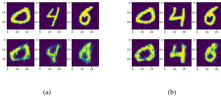
Fig. 3. Examples of MNIST images reconstructed by the CVNN before applying clustering. These images were encoded by the full transmitter scheme (including SHF and 64-IHQAM modulation), by considering a perfect channel: (a) Image reconstruction from 16 SHF coefficients, (b) Image reconstruction from 32 SHF coefficients.
