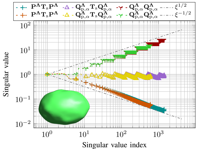
Fig. 5: Spectrum of the solenoidal part of the vector potential, its preconditioner, and its preconditioned counterpart. These spectra have been obtained for a smoothly-deformed sphere with a maximum diameter of 7.17 m (see insert), a frequency of 10^6 Hz, and for two different average edge lengths 0.31 m and 0.20 m. The spectra have been normalized so that their first singular value is one, for readability. Perfect filters built out of SVD have been used in these results.
