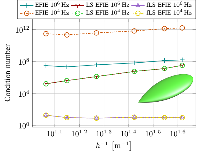
Fig. 4: Condition number of the EFIE (5), Loop-Star EFIE, and filtered Loop-Star EFIE (96) as a function of discretization for several frequencies. The condition number has been obtained after eliminating the isolated singular values, which have minimal impact on the convergence, arising from the deletion of one column from each of the preconditioning matrices. The solid lines correspond to a simulating frequency of 10^6 Hz and the dotted lines to a frequency of 10^4 Hz. The simulated structure is the NASA almond re-scaled to be enclosed in a bounding box of diameter 1.09 m. Perfect filters built out of SVD have been used in these results.
