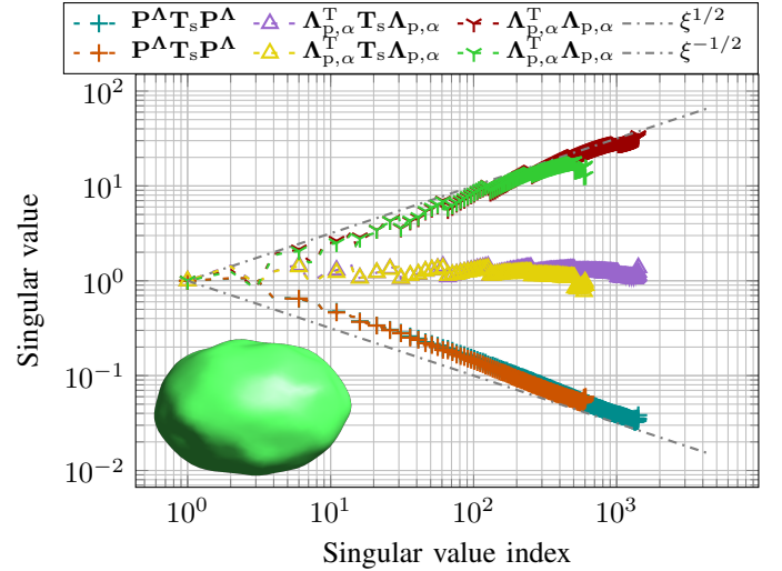
Fig. 2: Spectrum of the solenoidal part of the vector potential, its preconditioner, and its preconditioned counterpart. These spectra have been obtained for a smoothly-deformed sphere with a maximum diameter of 7.17 m (see insert), a frequency of 10^6 Hz, and for two different average edge lengths 0.31 m and 0.20 m. The spectra have been normalized so that their first singular value is one, for readability. Perfect filters built out of SVD have been used in these results.
