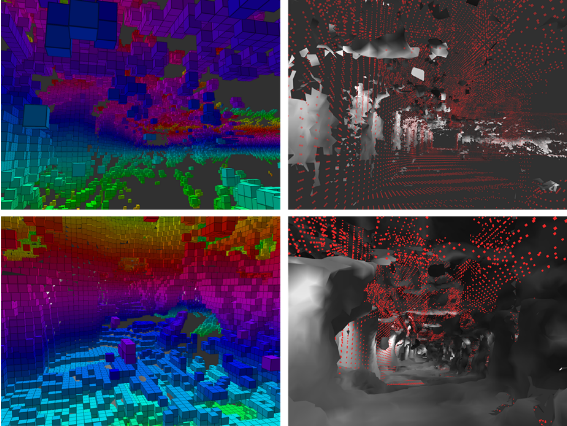
Figure 7. Multi-view volumetric fusion using Voxblox, 1 where the left image shows the voxel map, and the right image shows the 3D mesh reconstructed with marching cubes. The LiDAR measured point cloud is displayed in red for reference. The first line is the result on ORB-SLAM 3 11 estimated sparse depth. The second line is the predicted depth densified with our approach.
