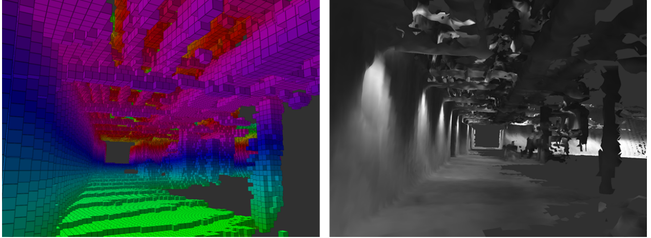
Figure 1. Multi-view mapping by Voxelblox 1 on the scene Basement_1 of HILTI SLAM Challenge Dataset. 2 The input data is a set of point clouds measured by a LiDAR sensor. The image on the left shows the constructed voxel map, and the image on the right is the textured 3D mesh deduced after application of marching cubes.
