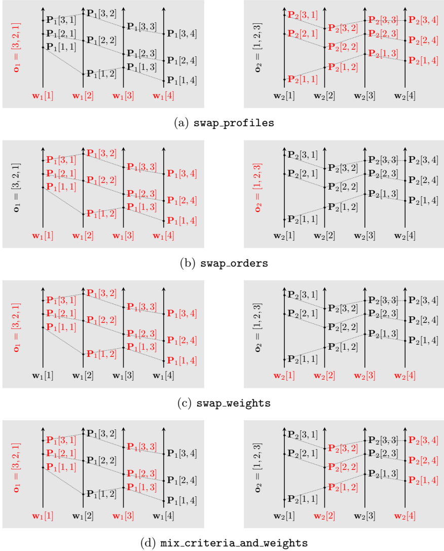
Fig. 2: Proposed crossover operators. Elements in red are assembled to build a child. Note that elements in black can also be assembled to produce a second child, as mentioned in Section 3 and done in our implementation.
