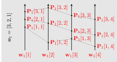
(a) swap_profiles
