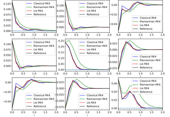
Fig. 2. Entries (i, j) of the covariance matrix across time for all schemes and the reference. On diagonal terms, the blue line cannot be crossed (this would result in a negative variance).
