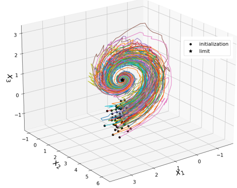
Fig. 1. 100 trajectories of the SDE (16) with our choice of parameters and a small time step (10 times larger than in the next figures).
