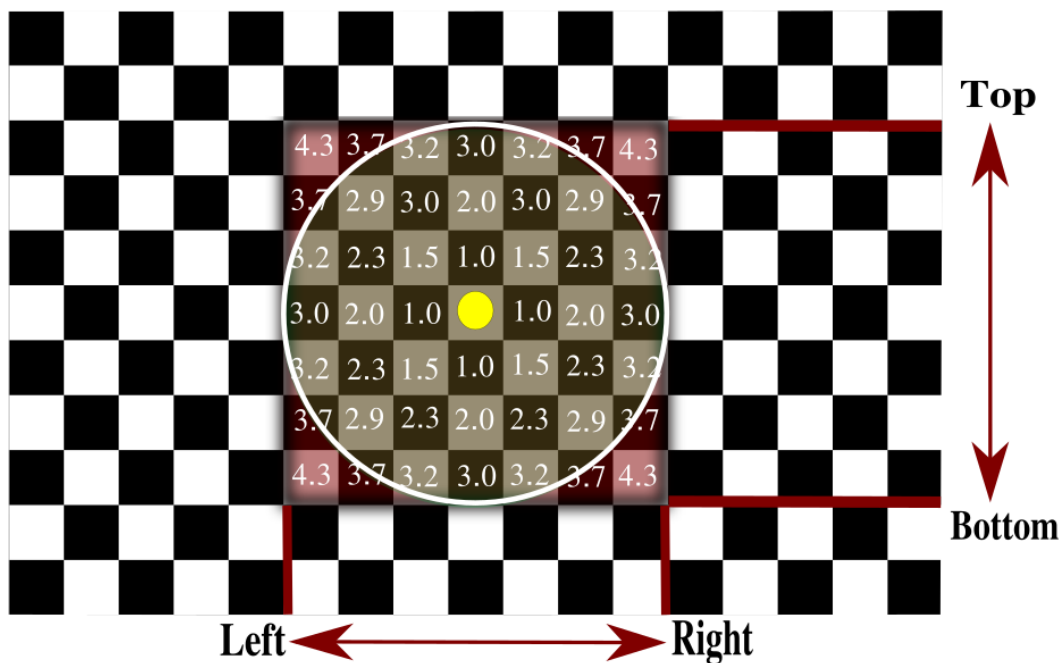
Figure 5: Random population using circle filling on a grid by bounding box
