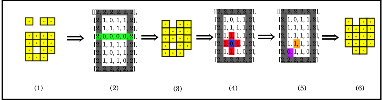
Figure 9: Compacity improver operator
