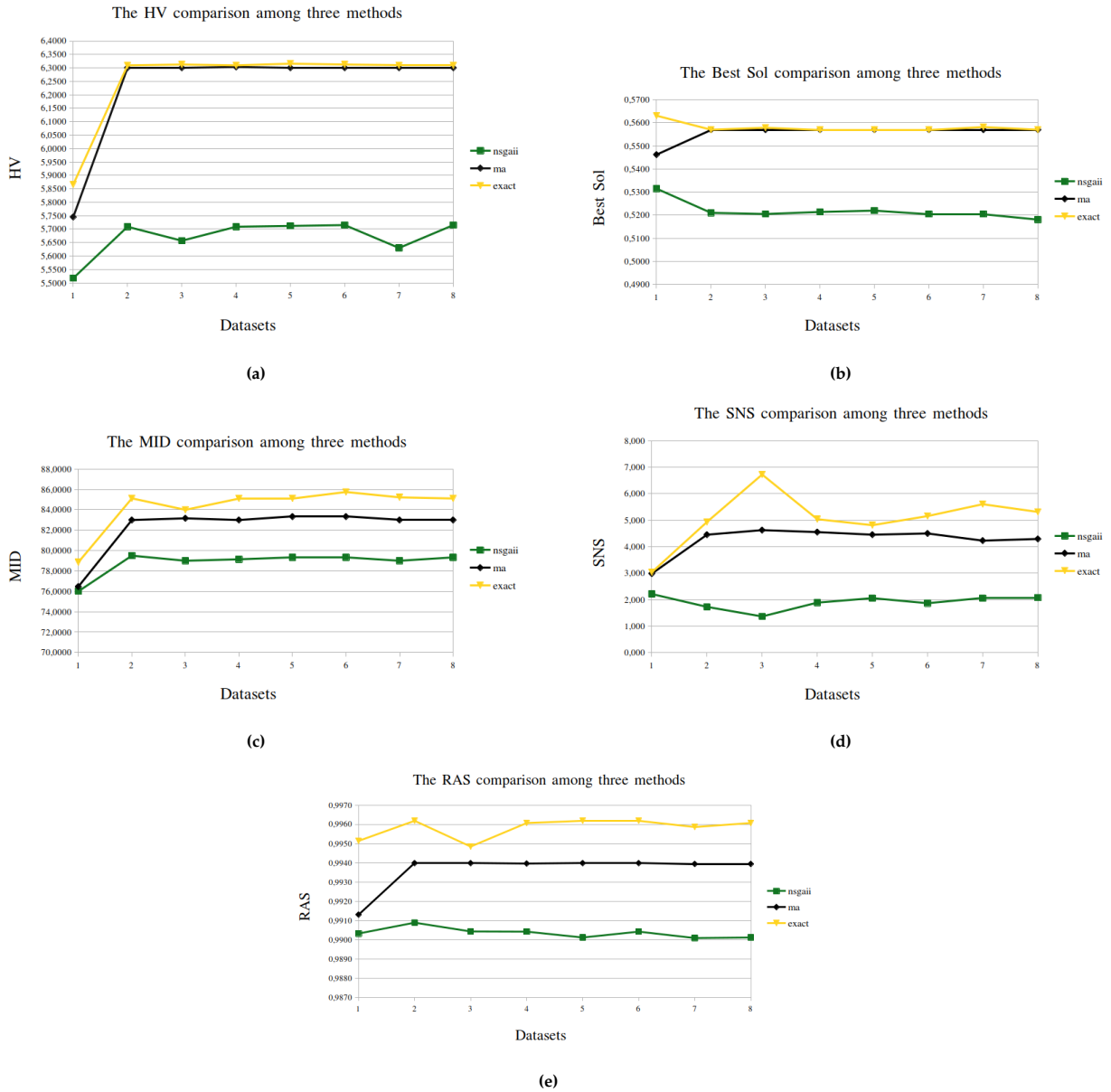
Figure 13: The comparison among MOEAs algorithms and exact optimal solutions for small size
