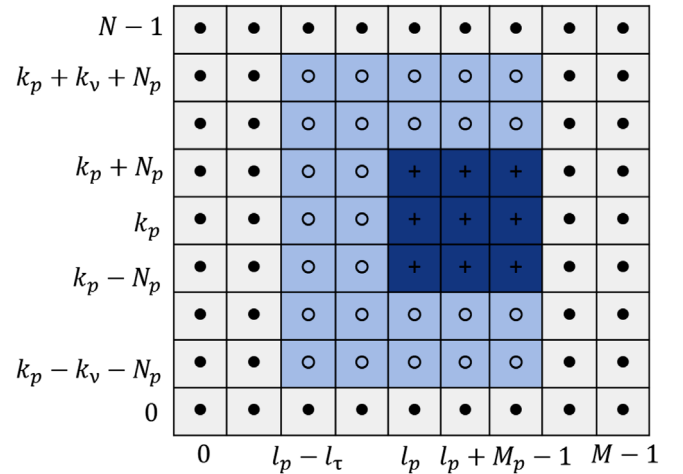
FIGURE 2 Symbol arrangement in the Delay-Doppler grid (+: pilot; •: data symbols; o: guard symbols)
