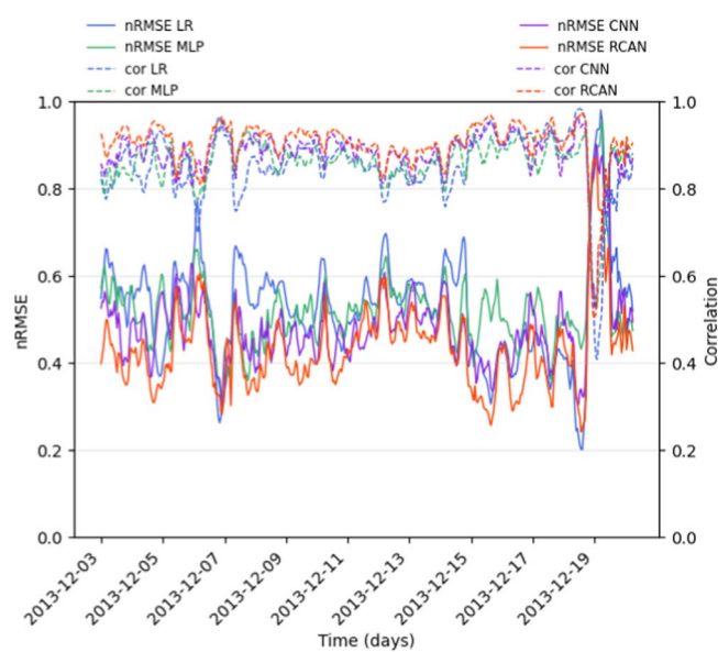
Figure A.2. \text{PM}_{10} nRMSE and correlation time series (a) of coarse resolution, pixel-based independent multi-layer perceptron (MLP), Convolutional neural network (CNN) and Residual channel attention network (RCAN) and summary statistics over the validation period as Taylor diagrams (b).
