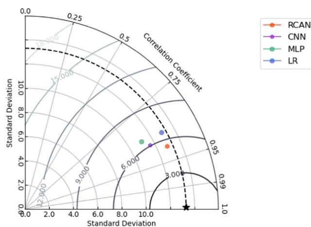
Figure A.3. \text{PM}_{10} summary statistics over the validation period as Taylor diagrams for low resolution simulation (LR), multi-layer perceptron (MLP), Convolutional neural network (CNN) and Residual channel attention network (RCAN) versus the high resolution (HR) considered as the 'truth'.
