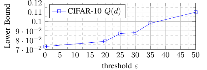
Fig. 4: Evolution of Q(D) on the dataset CIFAR10. \epsilon = 0 corresponds to Vanilla. \epsilon = 50 corresponds to classical Mixup .
