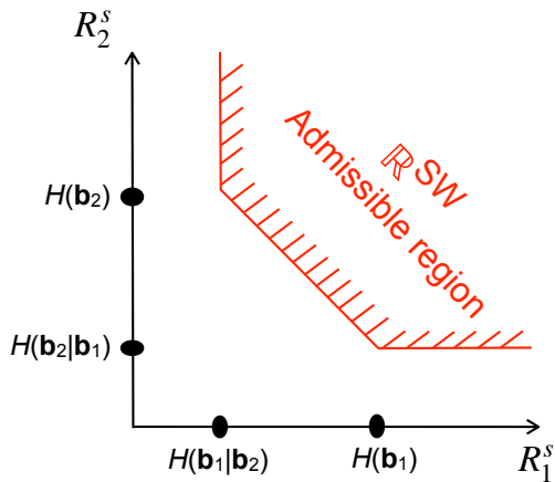
Fig. 2. Admissible region \mathbb{R}^{\text{SW}} specified with Slepian-Wolf theorem.
