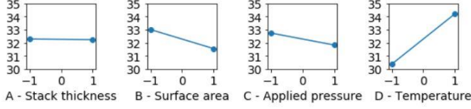
Fig. 7. Main effect plots for z-shrinkage.
