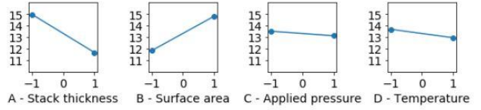
Fig. 9. Main effect plots for the combined x and y-direction shrinkage.
