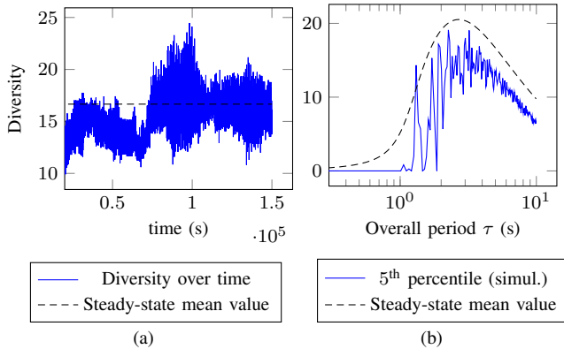
Fig. 4. Simulation versus theoretical results, with constant parameters for sensor arrivals and departures. One simulation trajectory of diversity over time is shown in (a), with the corresponding steady-state mean value for the Markovian model, for \tau = 5 . In (b) we compare the fifth percentile of simulated diversity with the theoretical mean diversity: both reach their maximum for approximately the same global period \tau .
