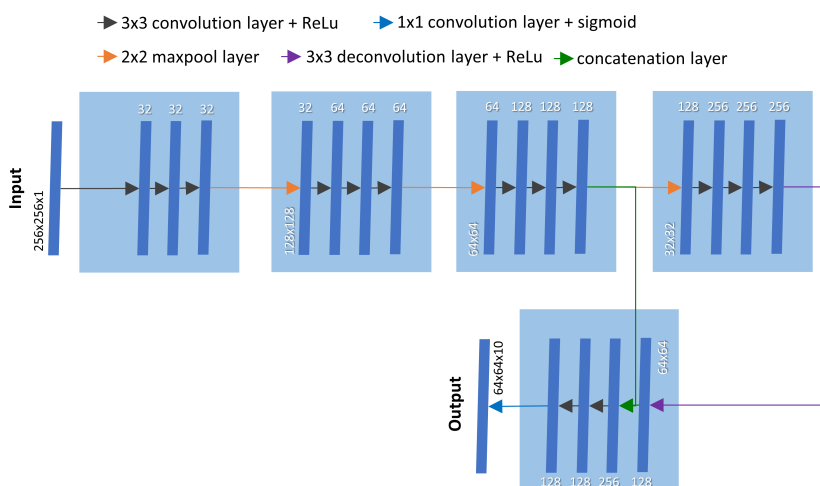
Figure 2. Architecture of the fully-supervised model. It is a UNet model [9] with a input shape fourfold the output to account for the imprecision of the annotation.
