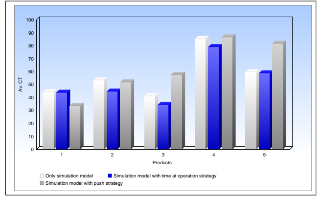
Fig. 4: Comparison of Av. CT between simulation and the two global scheduling strategies
