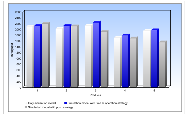
Fig. 5: Comparison of Throughput between simulation and the two global scheduling strategies
