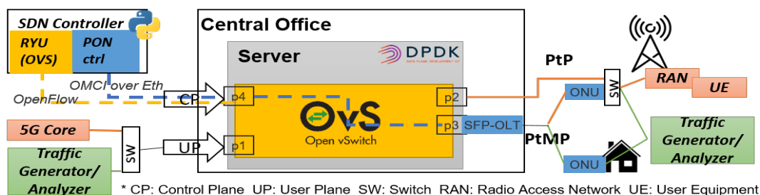
Fig. 2: Experimental setup
