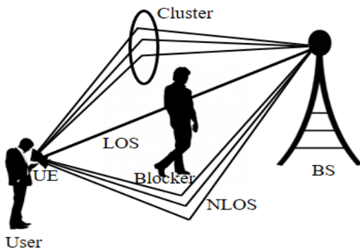
Fig. 6. Non-self-blocking illustration.
