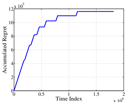
Fig. 4: Accumulated regret as a function of time for K = M = 4 .
