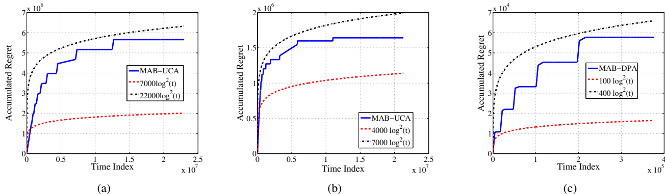
Fig. 3: Accumulated regret as time progresses (a) for the channel allocation phase with a constant exploration phase length, (b) for the channel allocation phase with a decreasing exploration phase length, (c) for the power allocation stage.
