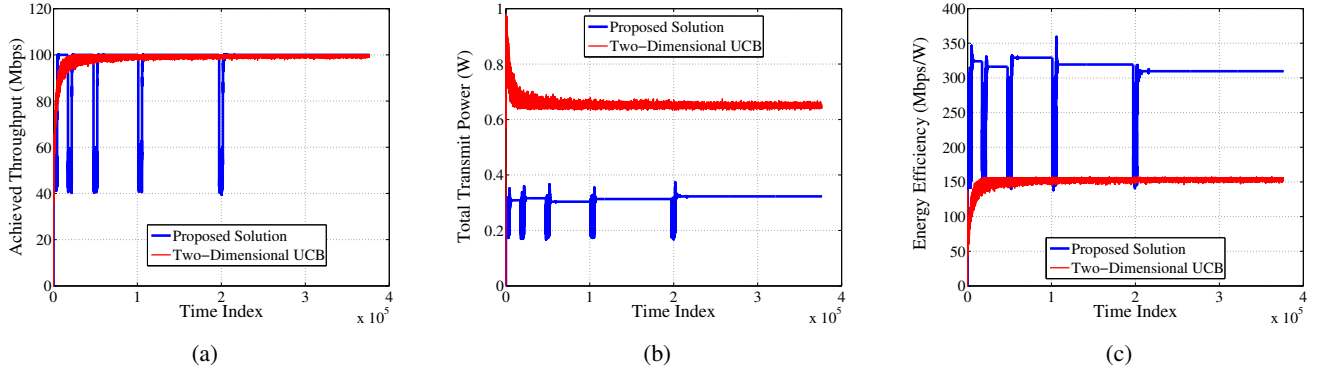
Fig. 5: Performance comparison as a function of time of (a) the achieved rate, (b) the total transmit power, (c) the energy efficiency.
