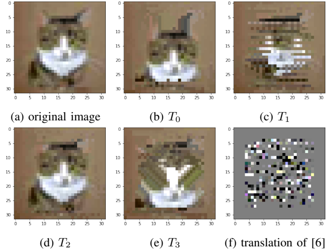
Fig. 3: Inferred translations T_0, T_1, \dots, T_3 and comparison with the translation defined in [6] on a near-regular graph.
