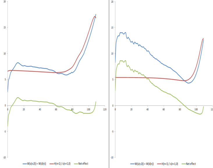
Figure 2: Effect of a variation of d_n on H_0 as a function of the age n , French men.
