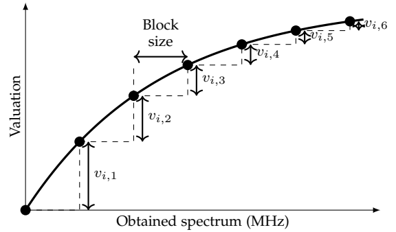
Figure 2: An example of a concave valuation function of obtained spectrum
