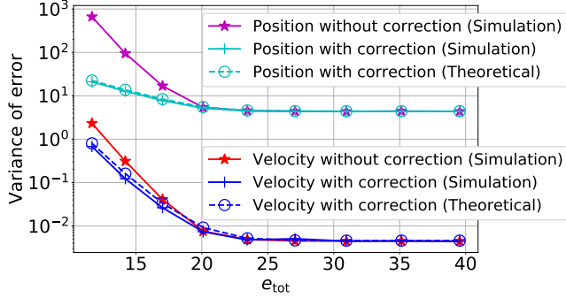
Fig. 1. Comparison between the simulated and theoretical variance of the estimation error at step N = 250 using the updated filter equations from Section 3.2 and the conventional equations both on a unreliable system.
