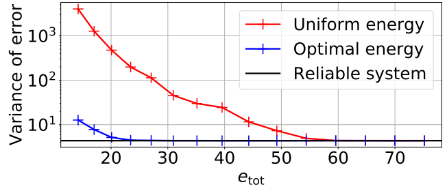
Fig. 2. Comparison of the variance of the total estimation error of the position at step N = 250 between using a uniform allocation of the energy across the bits and using the optimal allocation (16).
