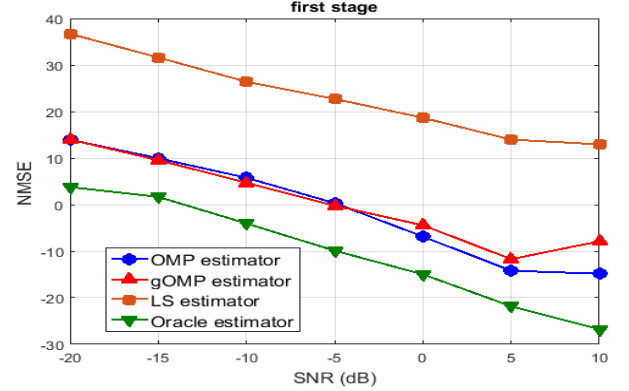
Fig. 2. NMSE performance of estimated at the first stage v.s. SNR for the LS, OMP, gOMP, and Oracle estimators
