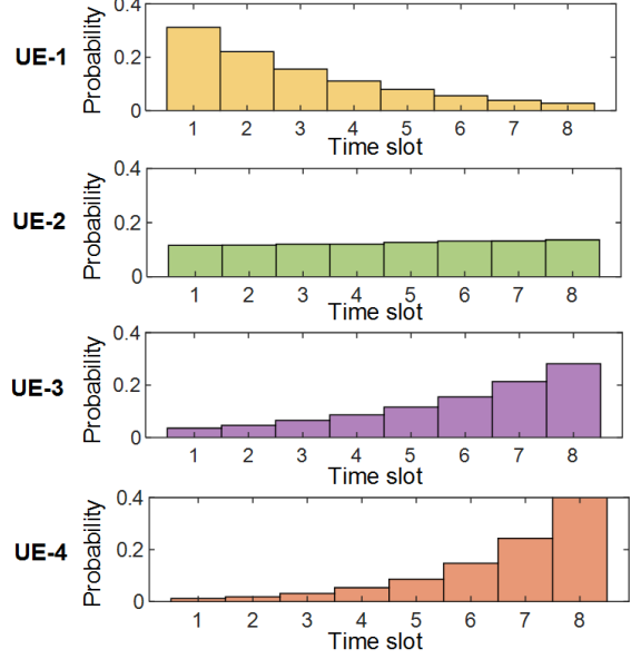
Fig. 4. PMFs of the time slot choice in a network with four relay candidates, R_d = 300 meters, b = 0.6 , shadowing \sigma_{dB} = 8 dB, and W = 8 time-slots. UE-1, UE-2, UE-3, and UE-4 are located 30, 120, 210, and 300 meters from the MTD, respectively.
