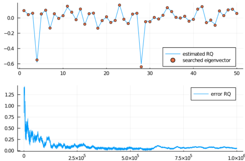
Fig. 2. Tracking with random walk exploration.
