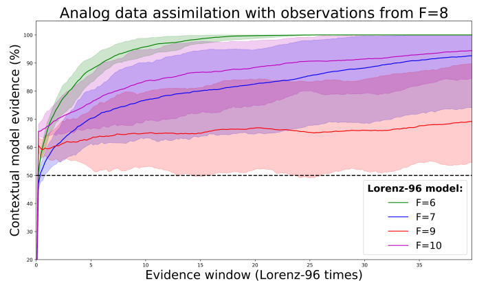
Fig. 1. Percentage of model evidence as a function of the evidence window. Observations are coming from the Lorenz-96 model, with forcing term F = 8 , and using an additive Gaussian noise with unit variance. The observations are compared to other Lorenz-96 models, using F = 6 to F = 10 . The procedure has been repeated on 10 independent observation sets to get an estimate of the confidence interval.
