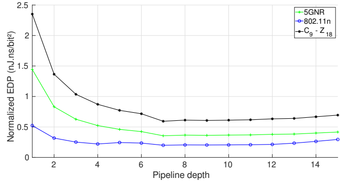
Fig. 4. Normalized EDP for different pipeline depths and codes, for a FER target of 10^{-2} at (E_b/N_0)_{WF} values (given in Table I).
