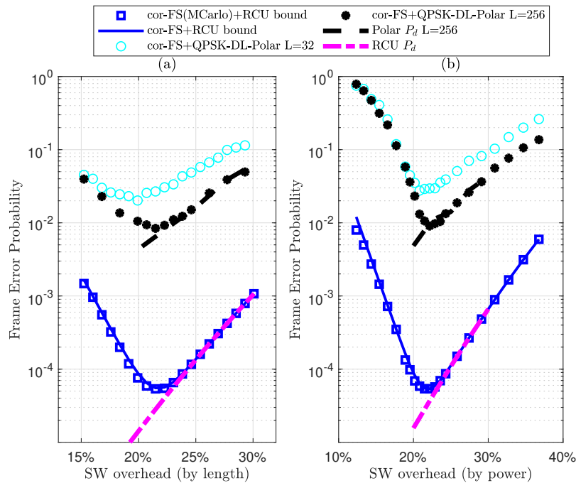
Fig. 5: CSW. P_E vs. SW overhead at frame length N = 256 and SNR \rho_t = -2\text{dB} with (a) uniform transmit power \rho_s = \rho_c but varying SW length m , or (b) fixed SW length m = 55 but varying SW-codeword power ratio. The continuous blue curves are P_{E,u} (5), the square curves are P_E (1) and the Polar-code curves are FEP.
