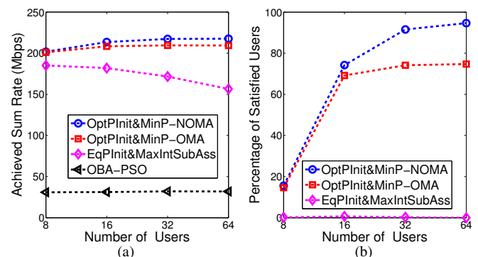
Fig. 4: Achieved sum rate (a), and percentage of satisfied users (b), in terms of K for R^{\text{req}} = 220 Mbps, P_{UAV}^{\max} = 1W and P_{MBS}^{\max} = 4W .
