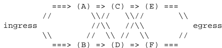
Figure 5: Packet Replication
