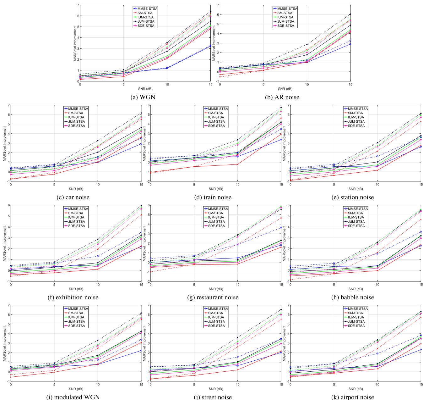
FIGURE 4. Speech quality evaluation by MARSovrl improvement after speech denoising using STSA-based methods for stationary, slowly-changing, speech-like and fast-changing non-stationary noise. As above, the dashed solid lines correspond to the performance measurements with known reference noise power spectrum, whereas the solid lines display the results obtained when the noise spectrum is estimated by B-E-DATE.
