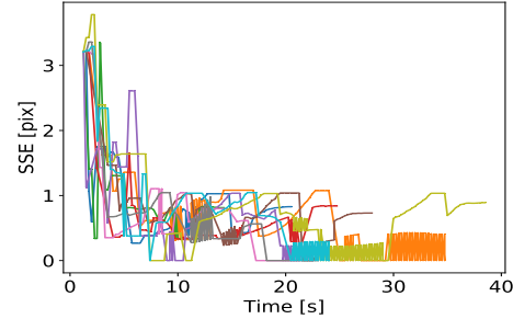
Fig. 5: Using the proposed LOD adaptation heuristic, the SSE of the object(s) in view quickly decreases below the target value.
